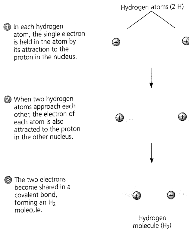
▲ Figure 2.7 Formation of a covalent bond.
