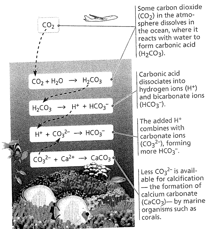
▲ Figure 2.24 Atmospheric CO_2 from human activities and its fate in the ocean.
