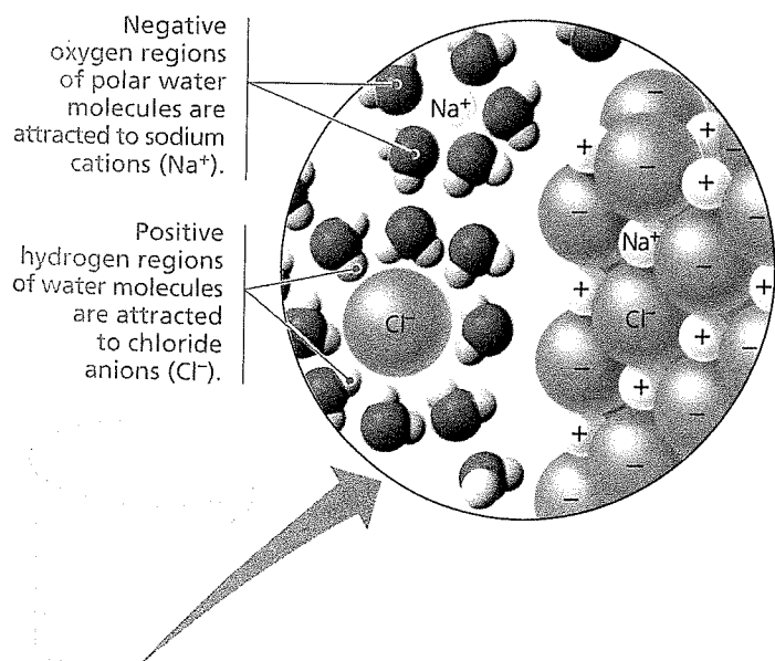
▲ Figure 2.21 Table salt dissolving in water. A sphere of water molecules, called a hydration shell, surrounds each solute ion.
