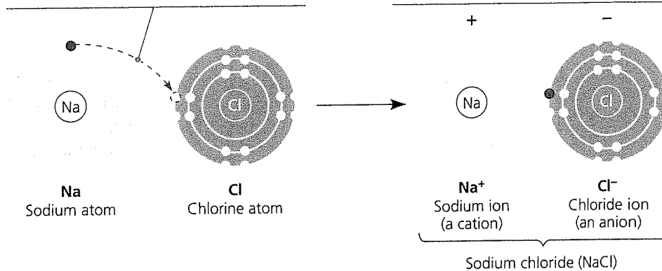
▲ Figure 2.10 Electron transfer and ionic bonding. The attraction between oppositely charged atoms, or ions, is an ionic bond. An ionic bond can form between any two oppositely charged ions, even if they have not been formed by transfer of an electron from one to the other.
